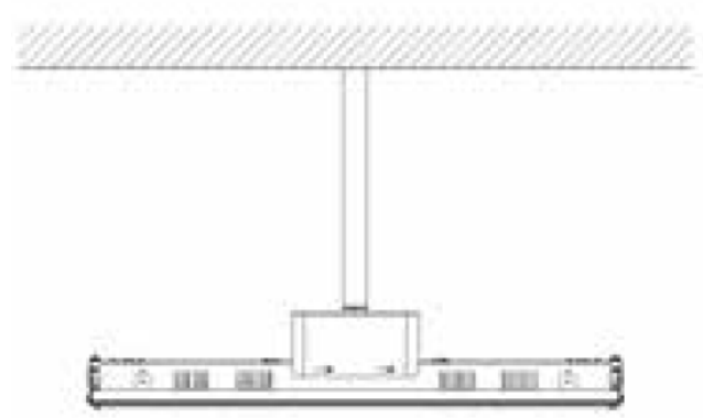
3/4" Pipe
